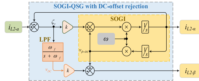
FIGURE 10 | ESOGI structure.
