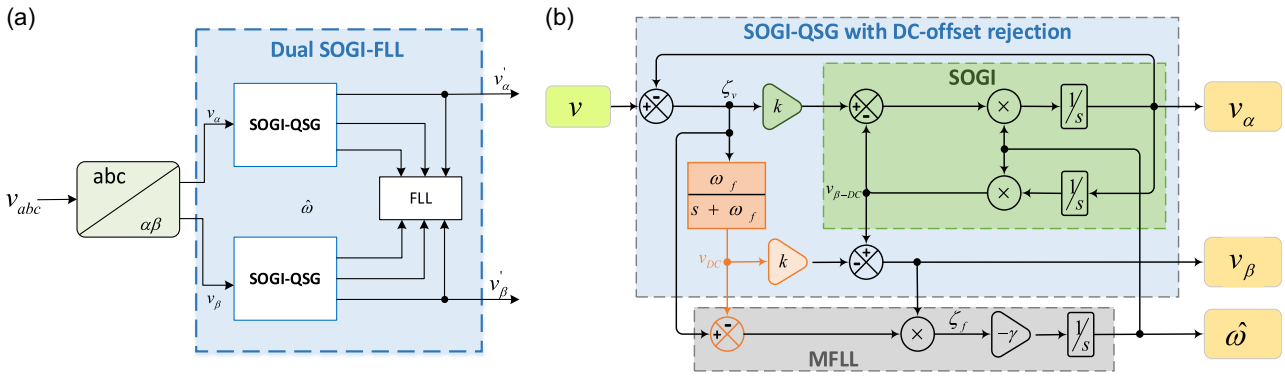
FIGURE 12 | The structure of (a) DESOGI-FLL and (b) ESGOGI-FLL.
