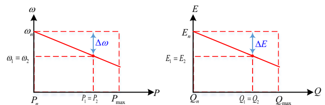
FIGURE 4 | Droop control characteristics.
