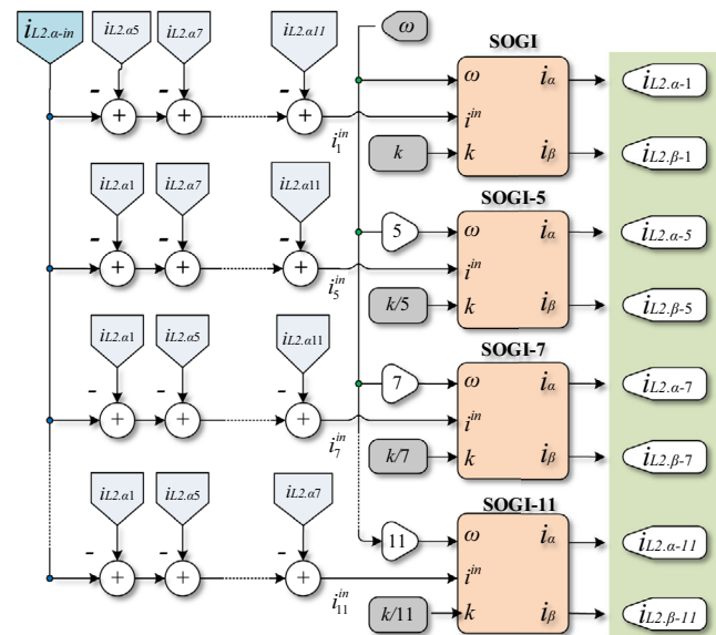
FIGURE 11 | Multiple-SOGI structure.
