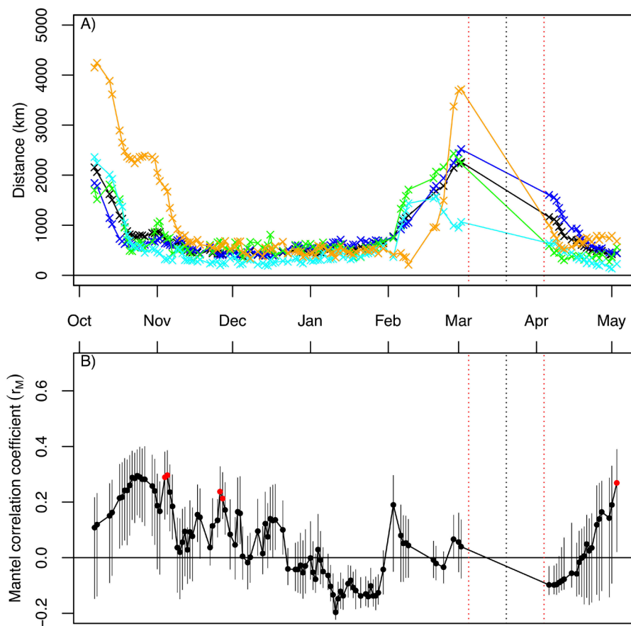
FIGURE 4 | Spatial structure of migrating and wintering adult American Golden-Plovers ( n=33 individuals) through time. (A) Non-breeding range spread of all individuals (variation in mean distances between individuals through time in black) and population spread for specific breeding population (dark blue: Bylot Island, light blue: Igloolik, green: Churchill, Orange: Alaskan populations); (B) Temporal variation in the Mantel coefficient ( r_M \pm 95\% confidence interval). Dates with significant positive r_M values are in red (permutation test, p < 0.05 ). Red vertical dashed lines indicate the periods with less reliable locations (i.e., obtained 15 days before and after the spring equinox, indicated by the black vertical dashed lines). Each tick mark is the first day of the month.
