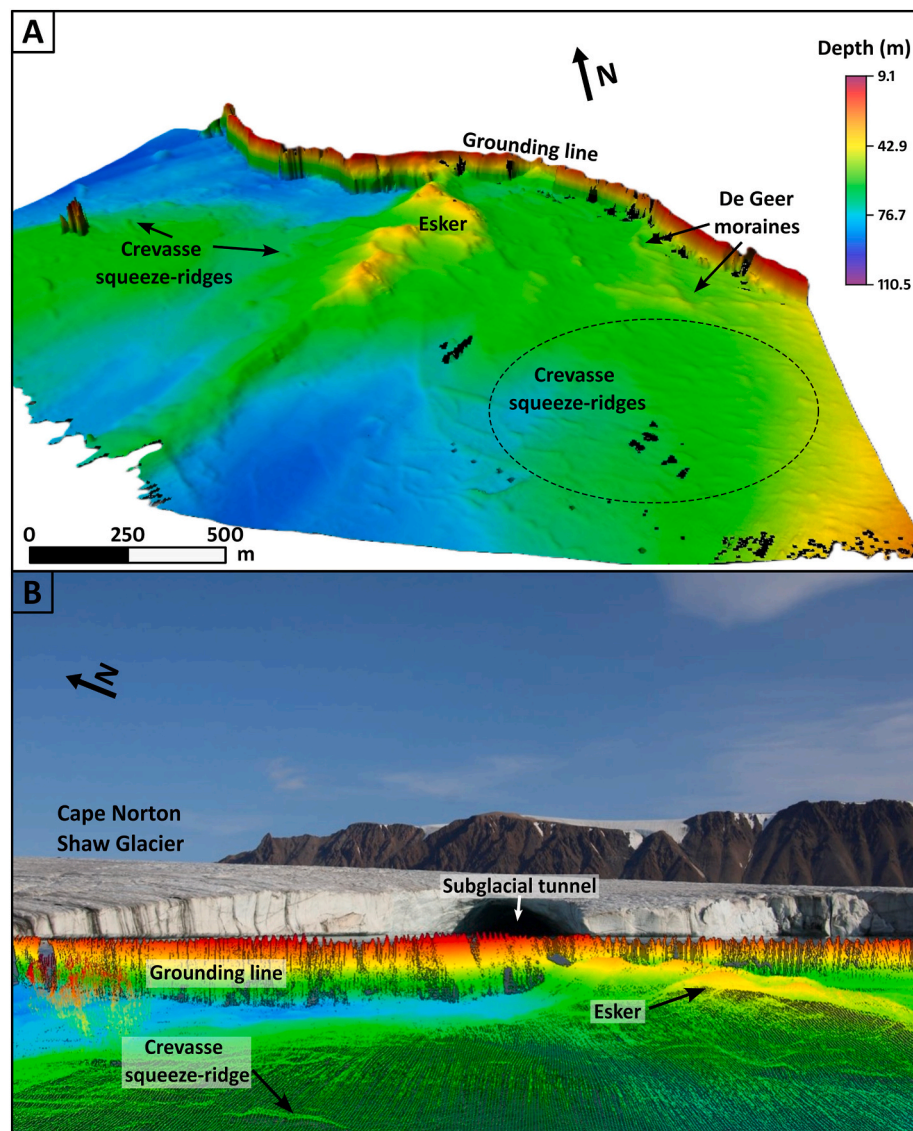
Fig. 4. (A) Bathymetric surface of an esker located close to the modern Cape Norton Shaw Glacier front with swarms of crevasse squeeze-ridges on both sides. (B) Photograph of the 2019 Cape Norton Shaw Glacier front showing the spatial relationship between the tunnel and the position of the esker in 2019. Location of the figure is provided on Fig. 2A. (For interpretation of the references to color in this figure legend, the reader is referred to the Web version of this article.)
