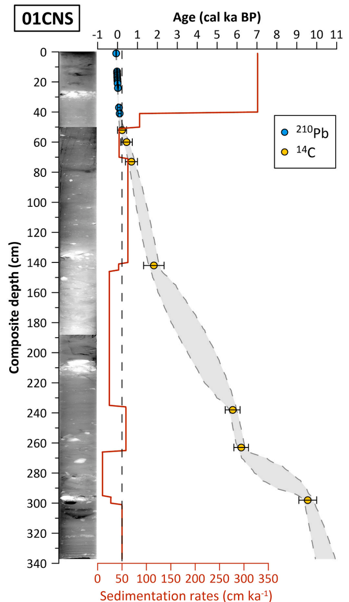
Fig. 8. Composite age-depth model for core 01CNS constructed using ^{210}\text{Pb} and ^{14}\text{C} ages. The Bayesian age-depth model was constructed using the R package rbacon (version 3.3.1; Blaauw and Christen, 2011). The gray shading represents the chronological uncertainties (95% confidence interval). The black dotted line represents the median of the data for the sedimentation rates. The estimated sedimentation rates in \text{cm ka}^{-1} are also shown. (For interpretation of the references to color in this figure legend, the reader is referred to the Web version of this article.)
