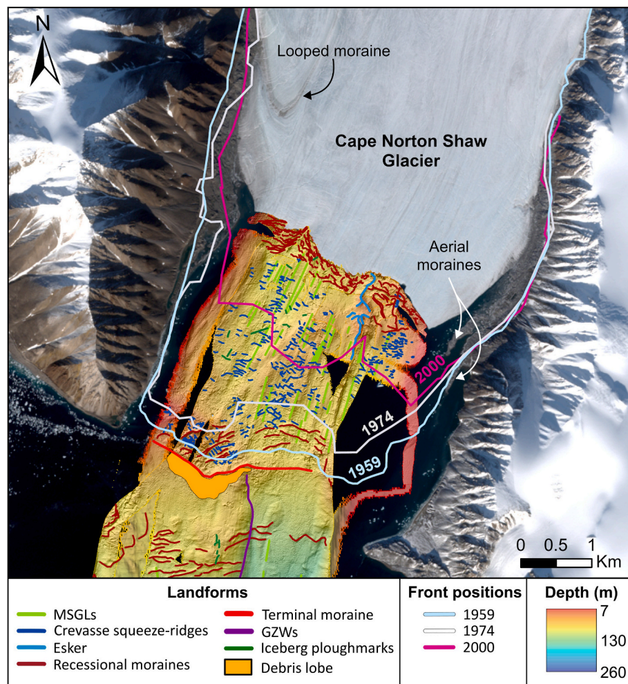
Fig. 12. Sentinel-2 image from 14 September 2023 (source: copernicus.eu) of the modern glacier front with swath bathymetric data from CCGS Amundsen and S/Y Vagabond . The colored lines represent the ice fronts in 1959 (light blue), 1974 (gray) and 2000 (pink). (For interpretation of the references to color in this figure legend, the reader is referred to the Web version of this article.)
