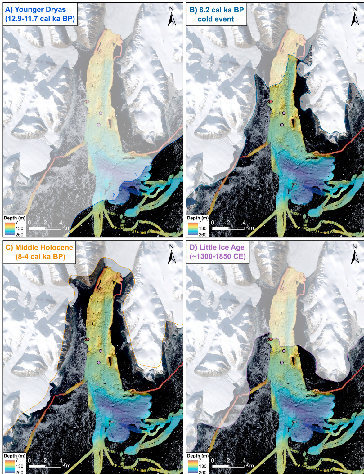
Fig. 11. Reconstruction of the ice extent over Cape Norton Shaw Inlet for the (A) Younger Dryas, (B) 8.2 cal ka BP cold event, (C) Middle Holocene (8-4 cal ka BP), and (D) Little Ice Age (~1300-1850 CE). Sentinel-2 image from 14 September 2023 (source: copernicus.eu) with swath bathymetric data from CCGS Amundsen and S/Y Vagabond . The ice-extent limits were modified from Dalton et al. (2023). (For interpretation of the references to color in this figure legend, the reader is referred to the Web version of this article.)
