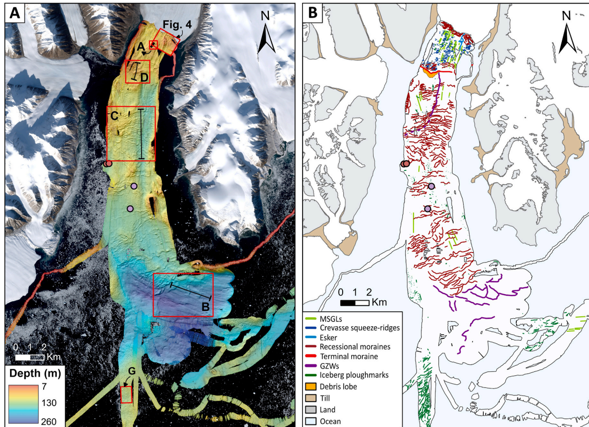
Fig. 2. (A) Swath bathymetry and 2023 Sentinel-2 satellite imagery (14/09/2023) of the modern glacier fronts in Cape Norton Shaw Inlet with cross profiles B-B', C-C' and D-D'. The red boxes show the locations of Fig. 3A, B, C, D and G close-ups and Fig. 4. The cores studied or cited in this paper are marked with circles: red for 33BC = AMD2303-33BC and 05GGC = AMD2303-05GGC, and purple for 02BC = AMD1803-02BC and 01 PC = AMD1803-01 PC (Stevenard et al., 2022). (B) Interpreted submarine landform distribution across the inlet. The color code follows the GlaciDat database from Streuff et al. (2022). (For interpretation of the references to color in this figure legend, the reader is referred to the Web version of this article.)
