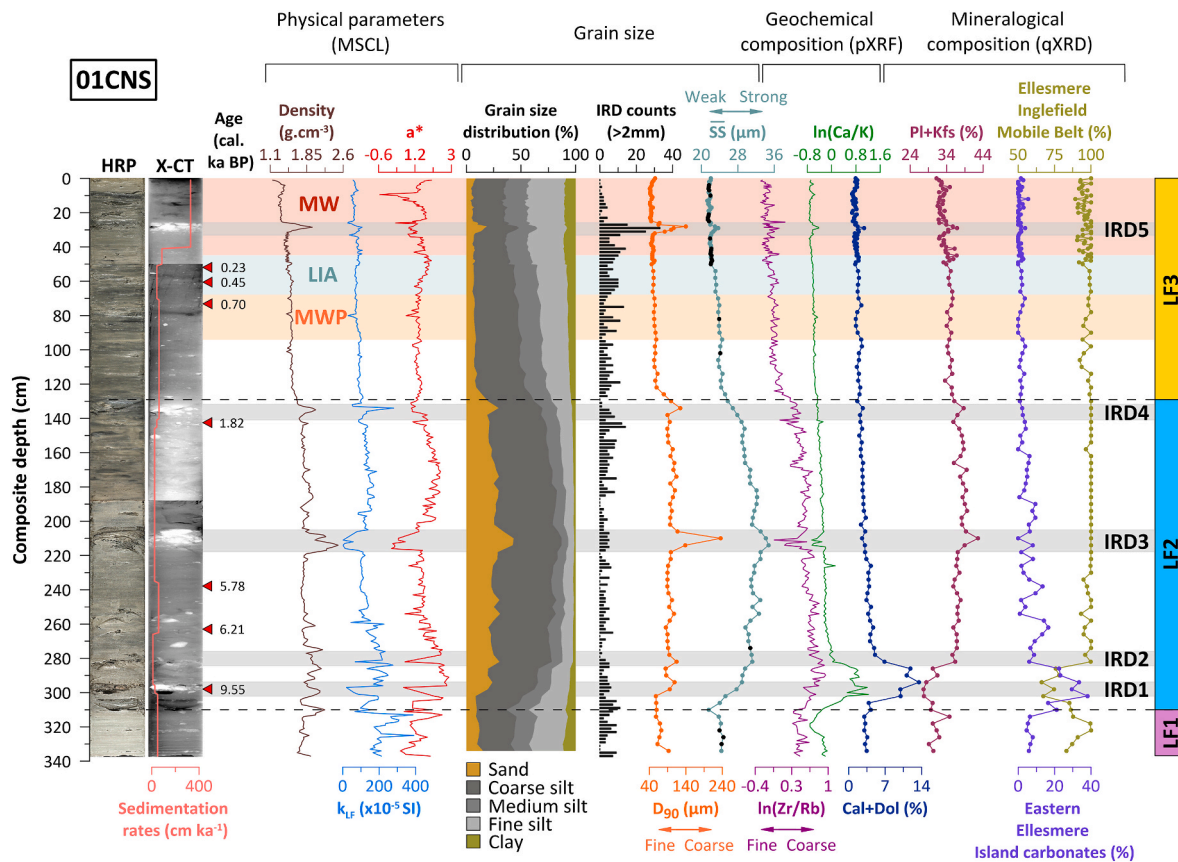
Fig. 7. High-resolution core photography, X-CT image, sedimentation rates, magnetic susceptibility ( k_{LF} ), a^* , grain size distribution, IRD counts (>2 mm fraction), D_{90} ( \mu\text{m} ), mean size of sortable silt fraction ( SS ), chemical and mineralogical tracers, SedUnMix results with the proportions of sediment from Eastern Ellesmere Island carbonates (purple) and Ellesmere-Inglefield Mobile Belt (green), and sedimentary units. The red triangles represent the radiocarbon dates. IRDs are numbered and highlighted in gray boxes. Black dots on the SS curve represent samples that do not pass the reliability test of a downcore correlation coefficient >0.5 between SS and SS\% . MW: Medieval Warming, LIA: Little Ice Age, MW: Modern Warming. (For interpretation of the references to color in this figure legend, the reader is referred to the Web version of this article.)
