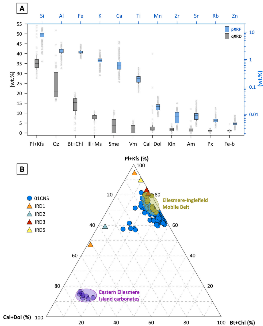
Fig. 6. (A) Boxplot of the chemical (pXRF) distributions of the main elements (wt.%; blue) and the mineralogical (qXRD) distributions of the main minerals (wt.%; gray) within the composite core. Note that the relative concentrations obtained with the pXRF sensor were converted to percentages (1% = 10,000 ppm) for better visualization. (B) Mineralogical ternary plot of plagioclase + K-feldspar (Pl+Kfs) – biotite + chlorite (Bt+Chl) – calcite + dolomite (Cal+Dol) for cores O1CNS (this study) and O1 PC (Stevenard et al., 2022). The source data for eastern Ellesmere Island carbonates (purple circles) are from Bicera-Nfundiko (2024), and those for the Ellesmere-Inglefield Mobile Belt (green circles) are from Stevenard et al. (2022). (For interpretation of the references to color in this figure legend, the reader is referred to the Web version of this article.)
