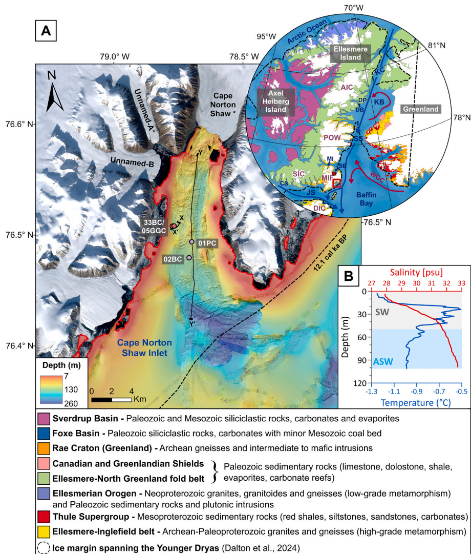
Fig. 1. (A) Map of Cape Norton Shaw Inlet. A Sentinel-2 image acquired on 14 September 2023 (Copernicus.eu) is overlain by the IBCAO topobathymetric map (Jakobsson et al., 2020) and swath bathymetric data collected by the CCGS Amundsen and the S/Y Vagabond . Cross-profiles X-X' and Y-Y' are presented in Fig. 5. The cores studied or cited in this paper are marked by circles: red for 33BC = AMD2303-33BC and 05GGC = AMD2303-05GGC, and purple for 02BC = AMD1803-02BC and 01 PC = AMD1803-01 PC (Stevenard et al., 2022); Asterisks (*) identify surge-type glaciers. The circular map shows the geological setting of northern Baffin Bay and the major surface currents (Harrison et al., 2015). The red arrows represent warm surface currents ( >2^\circ\text{C} ), and the blue arrows represent cold Arctic Surface Water (ASW) ( <-1^\circ\text{C} ). Dashed line indicates the Younger Dryas (~12.1 cal ka BP) optimal ice margin (Dalton et al., 2024). Red circle represents Mittie Glacier. WGC = West Greenland Current; CS=Cape Storm; DB=Dobbin Bay; DP=Darling Peninsula; JS=Jones Sound; KB=Kane Basin; KC=Kennedy Channel; MI=Makinson Inlet; SB=Smith Bay; SS=Smith Sound; AIC=Agassiz Ice Cap; DIC=Devon Ice Cap; MIF=Manson Icefield; POW=Prince of Wales Icefield; SIC=Sydkap Ice Cap. (B) Temperature and salinity profiles from CTD casts taken during the 2023 Amundsen expedition at the core locations of 33BC-05GGC (24.09.2023). SW: Surface Water and ASW: Arctic Surface Water. (For interpretation of the references to color in this figure legend, the reader is referred to the Web version of this article.)
