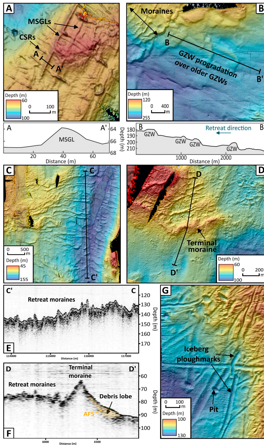
Fig. 3. Close-ups of submarine landforms in Cape Norton Shaw Inlet. (A) Examples of mega-scale glacial lineations (MSGLs) and crevasse squeeze-ridges (CSRs) landforms and cross-section profile A-A' across a mega-scale glacial lineation. (B) Examples of grounding zone wedges (GZW) and retreat moraine landforms with cross-section profile B-B' across prograding grounding zone wedges. (C) Examples of De Geer moraines with the cross-section profile C-C' associated with the seismic profile (E). (D) Examples of the 1959 terminal moraine, debris lobe and De Geer moraines with cross-sectional profile D-D' associated with the seismic profile (F). (G) Examples of iceberg ploughmarks and pits at the mouth of the inlet. (For interpretation of the references to color in this figure legend, the reader is referred to the Web version of this article.)
