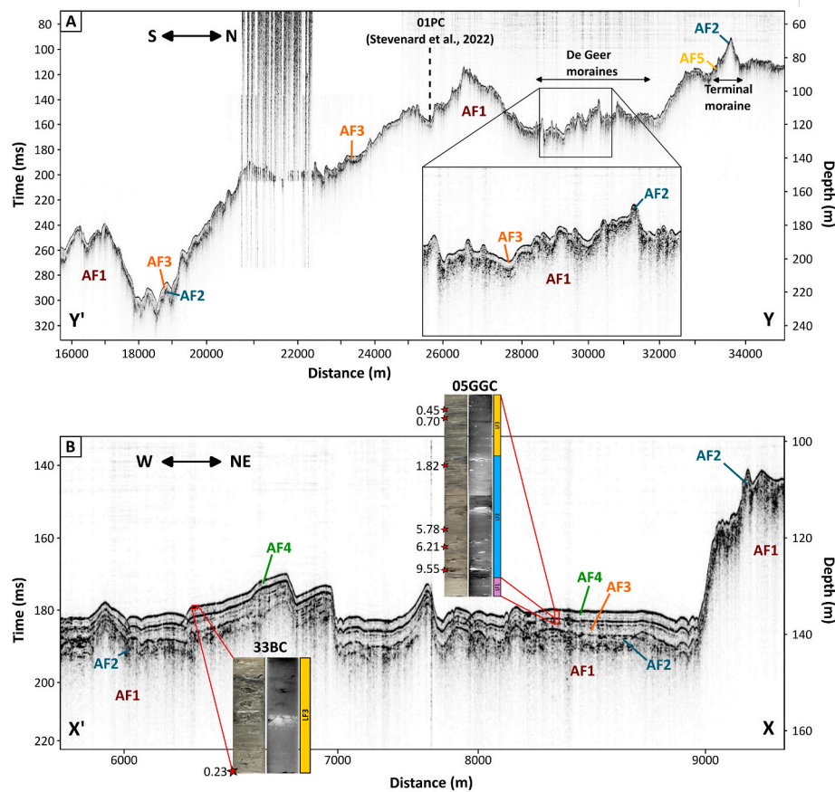
Fig. 5. Acoustic sub-bottom profiles across Cape Norton Shaw Inlet with interpreted units. The locations of the profiles are shown in Fig. 1. (A) Sub-bottom profile Y'-Y of lines 211-0957 acquired in 2017, showing the approximate locations of core 01 PC (Stevenard et al., 2022) and four acoustic facies (AF1-AF3 and AF5). (B) Sub-bottom profile X'-X of lines 267-1412 acquired in 2023, showing the approximate locations of cores 33BC and 05GGC and the acoustic facies AF1-AF4. The red stars in the figure indicate ages in cal yr BP. (For interpretation of the references to color in this figure legend, the reader is referred to the Web version of this article.)
