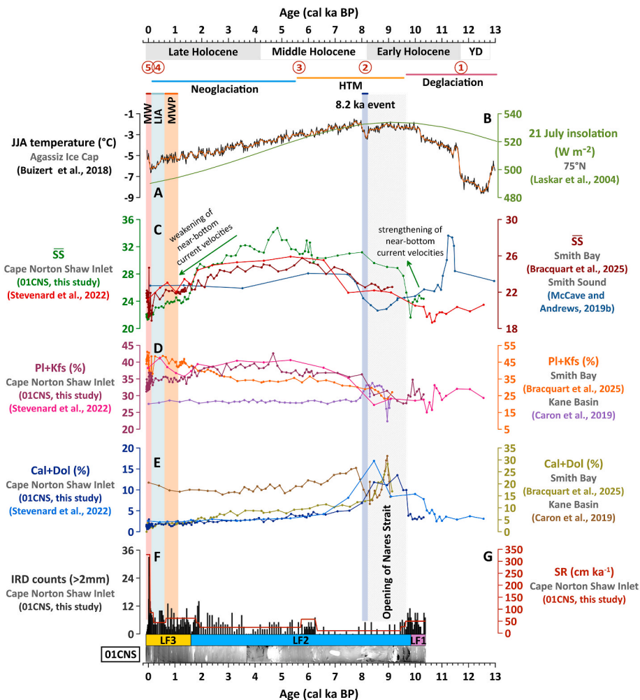
Fig. 9. Comparison of proxies used in this study (01CNS) with paleoenvironmental proxies. (A) Reconstructed summer temperature ( ^{\circ}\text{C} ) of the Agassiz Ice Cap (Buziert et al., 2018). (B) 21 July insolation at 75^{\circ}\text{N} (Laskar et al., 2004). (C) Mean size of sortable silt fraction ( \overline{SS} ) from cores 01CNS (green, this study), 01MCS (dark red, Bracquart et al., 2025), AMD1803-01 PC (red, Stevenard et al., 2022) and 2001LSSL-014PC (blue, McCave and Andrews, 2019b). (D) PI + Kfs (%) from cores 01CNS (crimson, this study), 01MCS (orange, Bracquart et al., 2025), AMD1803-01 PC (pink, Stevenard et al., 2022) and AMD14-Kane2B (purple, Caron et al., 2019). (E) Cal + Dol (%) from cores 01CNS (dark blue, this study), 01MCS (green, Bracquart et al., 2025), AMD1803-01 PC (light blue, Stevenard et al., 2022) and AMD14-Kane2B (gold, Caron et al., 2019). (F) IRD count ( >2\text{mm} ), and (G) sedimentation rates ( \text{cm ka}^{-1} ) from cores 01CNS (this study). #1 to #5 indicates conditions shown in Fig. 10A–E. (For interpretation of the references to color in this figure legend, the reader is referred to the Web version of this article.)
