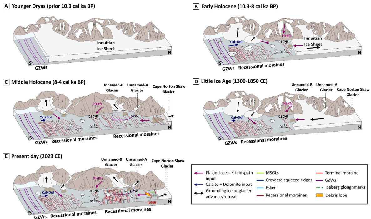
Fig. 10. Reconstruction of the sedimentary processes and environmental conditions in Cape Norton Shaw Inlet during the: (A) Younger Dryas (prior to 10.3 cal ka BP), (B) early Holocene (10.3–8 cal ka BP), (C) middle Holocene (8–4 cal ka BP), and late Holocene (4 cal ka BP to present), with a distinction between (D) the Little Ice Age (LIA; ~1300–1850 CE) and (E) the present day (2023 CE).
