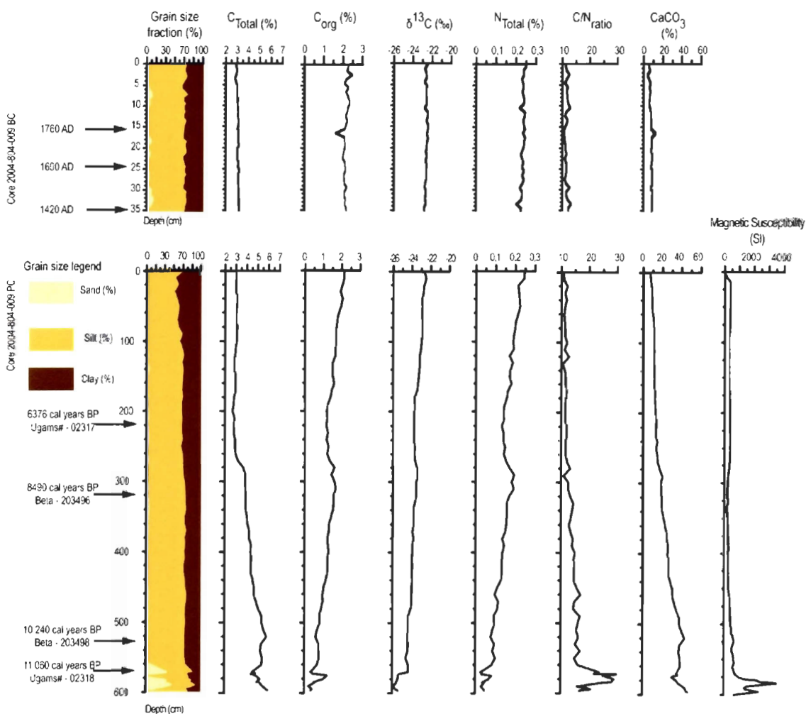
Figure 5. Sedimentological (grain size) and geochemical (stable isotopes) content of cores 2004-804-009 BC and 2004-804-009 PC. The chronology of core 2004-804-009 BC is estimated from ^{210}\text{Pb} measurements and expressed in years AD (Fig. 3). The chronology of core 2004-804-009 PC is estimated from accelerator mass spectrometry (AMS) ^{14}\text{C} dates on mollusc shells and mixed benthic foraminifers. It is expressed in calibrated years BP (Fig. 4).
