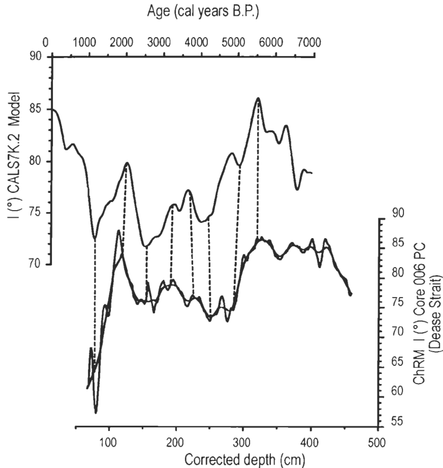
Figure 5. ChRM I for core 006 PC and magnetic inclination I ( ^{\circ} ) for Dease Strait inferred from the CALS7K.2 model. The dashed lines are the suggested correlations with the CALS7K.2 model [Korte and Constable, 2005].
