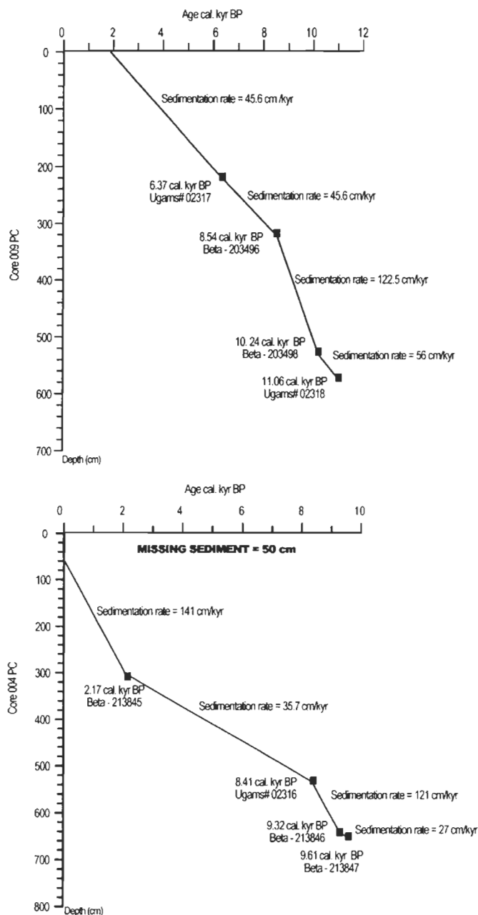
Figure 4b. (background data set). Initial age-depth model for cores 009 and 004 PC, respectively. Both age models are based on linear interpolation fit between calibrated AMS- ^{14}\text{C} and indicate sedimentation rates ranging from 45 to 122 cm/kyr and from 27 to 141 cm/kyr for cores 009 and 004 PC respectively. The grey zone corresponds to the missing sediment due to piston coring process.
