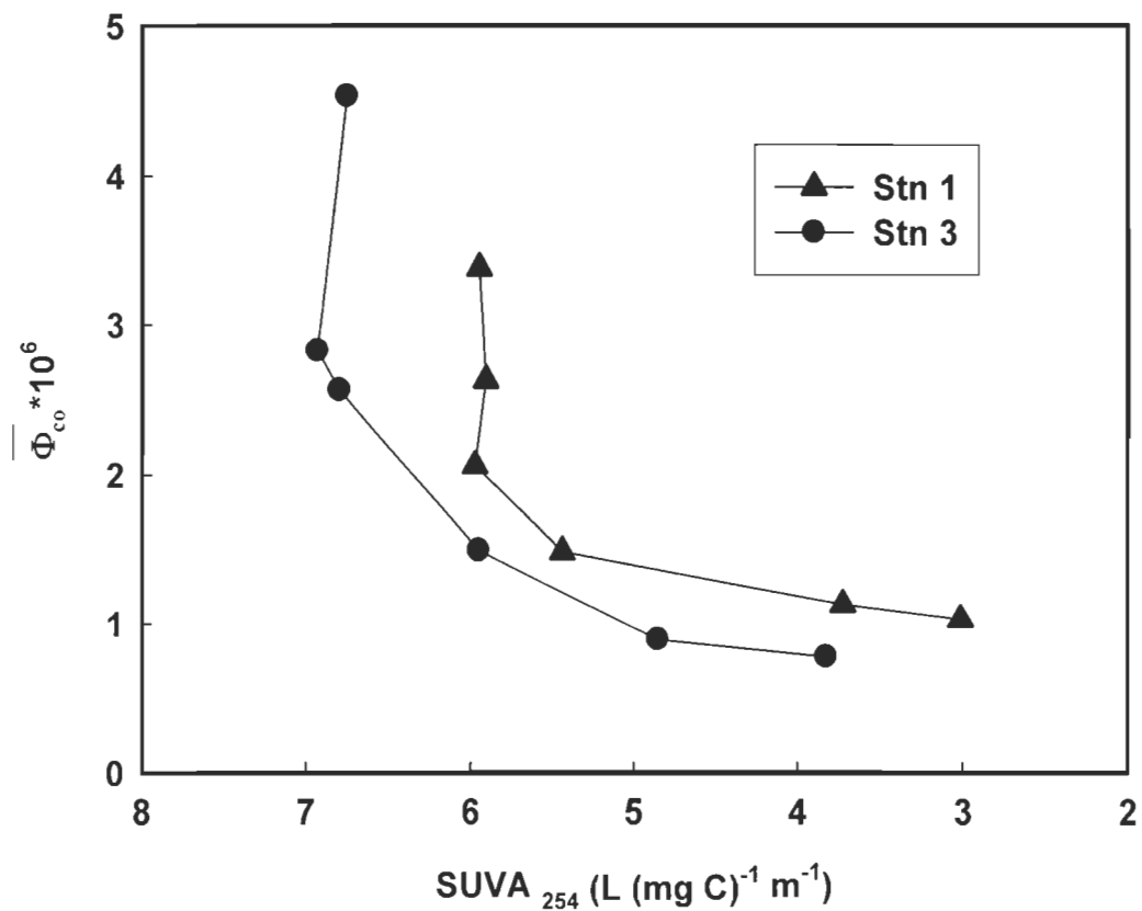
Figure 3-11. Effect of pre-fading on the CO quantum yields as illustrated by the plots of \bar{\Phi}_{CO} vs the specific absorption coefficient at 254 nm (Stns. 1 and 3 only; SUVA 254 data for the rest of the stations are not available).
