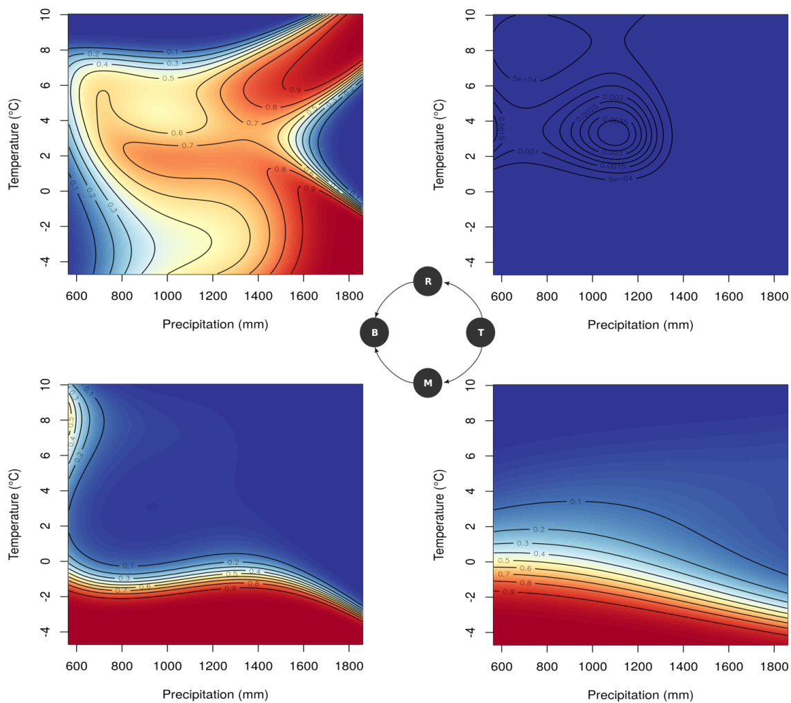
Figure S4: Transition probabilities of all pathways from (T)emperate to (B)oreal. Each panel corresponds to one pathway which can be attached to one arrows of the centered STM diagram (presented in figure 1). Transition probabilities were estimated by multinomial regression accounting for the temperature ( ^{\circ}\text{C} ) on the y-axis and the precipitation (mm) on the x-axis.
