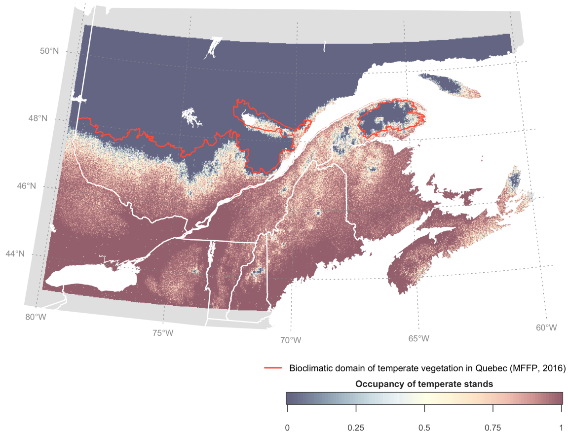
Figure S3: The STM predictions of the present extent of temperate forest (colour scale) is largely concordant with expert-drawn maps (provided by the forest ministry of Quebec; MFFP 2016) delineating the extent of the temperate forest bioclimatic domain (red line), although there is some disagreement at the transition. Projections were made using the STM with demographic, biotic, and dispersal constraints and show the proportion of simulations where temperate or mixed forest was present.
