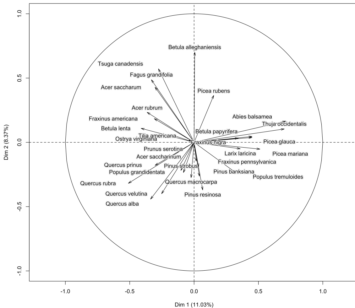
Figure S1: Principal component analysis of the first 30 dominant species (in terms of the basal area) in Eastern North America. This unconstrained ordination used site/species matrix, with Hellinger transformation. Data are represented in a Euclidean space. The first axis, representing 11% of the variance, illustrates the divergence in species composition among boreal and temperate communities.
