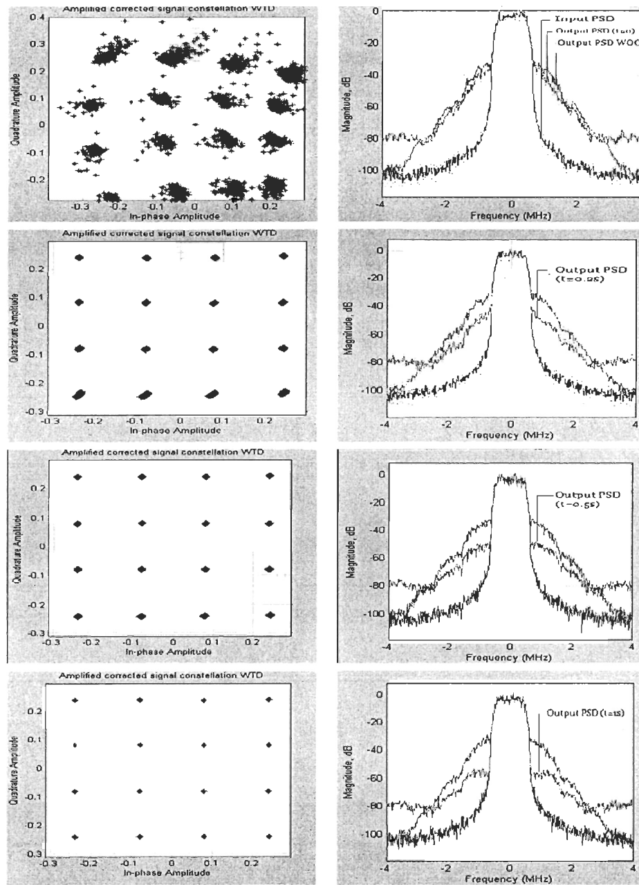
Figure 2.19: Output signal constellation and power spectral density during adaptation process ( t=0 s (Top), t=0.2 s and t=0.5 s (middle), and t=1 s (Bottom)).
