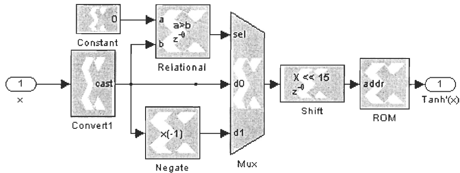
Figure 2.29: Implementation of the nonlinear activation function derivative.
