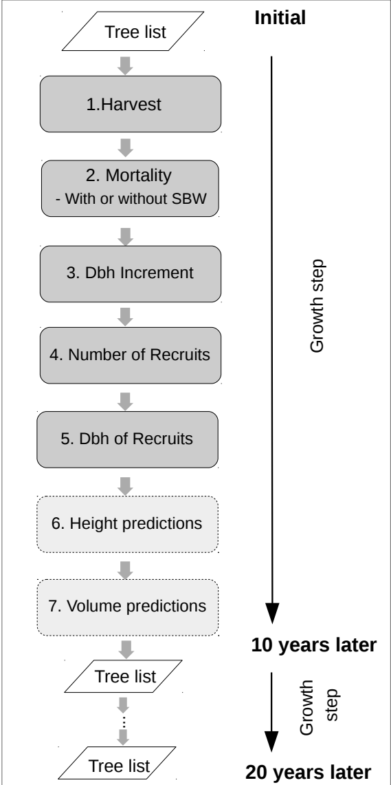
Figure 1: Flowchart of ARTEMIS-2009 considering its iterative process. Dark gray boxes represent the dynamic sub-models. Dotted light gray boxes are the static sub-models.
