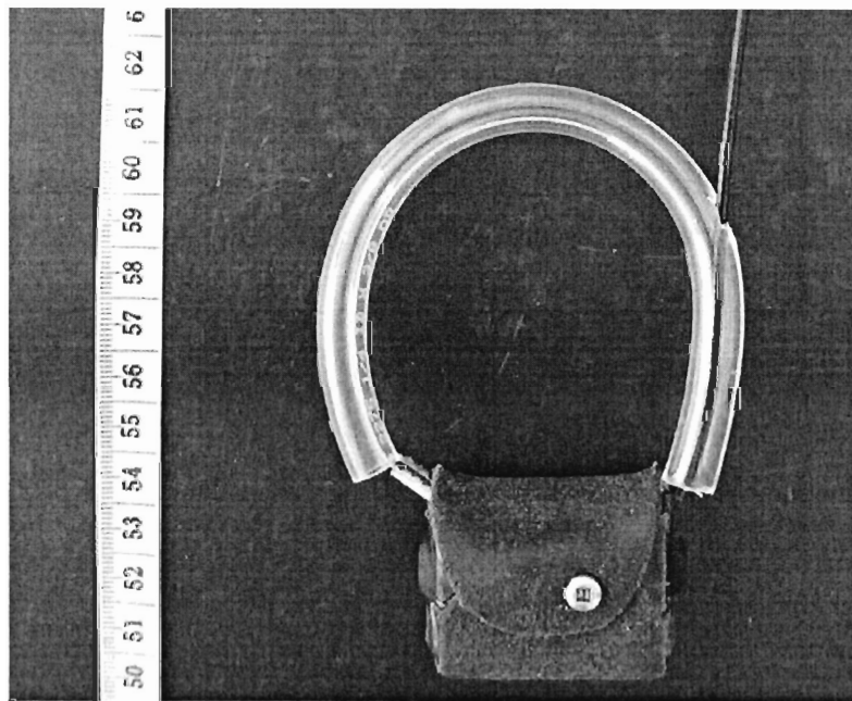
Figure 2.2 : Tygon tubing system used to attach radio transmitter to North American porcupines in Parc National du Bic, Québec, May 2000-May 2005. Note that the metallic part (cramp) used to close the collar is visible on the picture but was inserted into the Tygon after the collar was adjusted around the porcupine's neck. Photo by S. Descamps.
