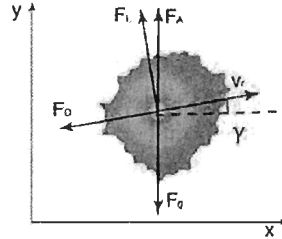
1. Fig. 1. Forces acting on the water droplet
