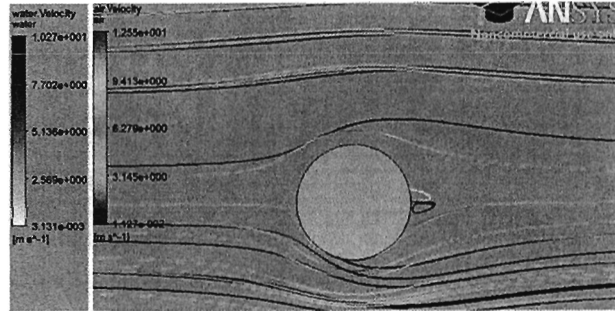
Figure 7: Air – water multiphase velocity simulation on CFX
