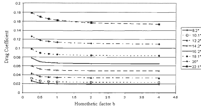
Figure 2: Drag coefficient vs. homothetic factor for different angles of attack
