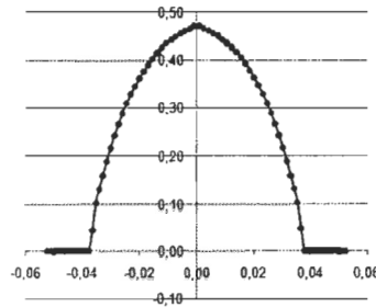
Figure 10: CFX Eulerian based Local collection efficiency distribution along circumference of cylinder
