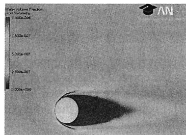
Figure 8: Illustration of the distribution of the water volume fraction
