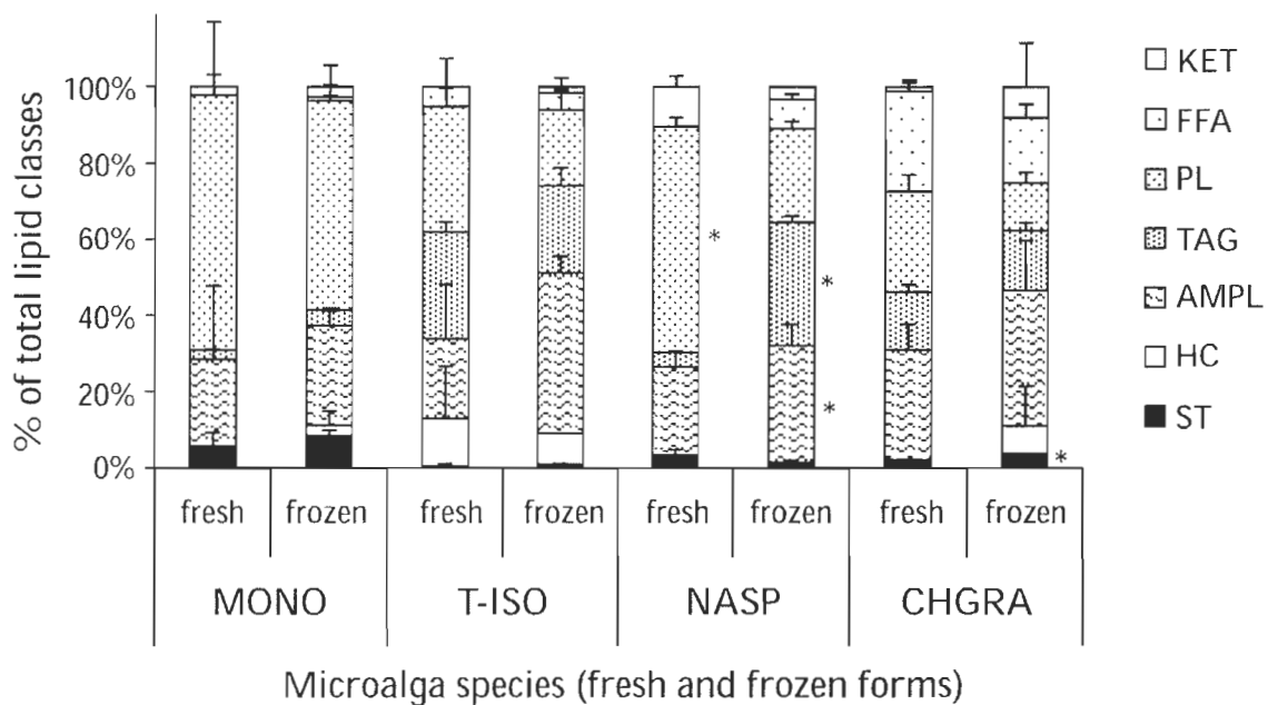
Figure II.1 Mean proportions of lipid classes \pm SD (% weight of total lipids) contained in fresh and frozen-concentrated microalgae. Asterisks indicate significant difference between the two forms. KET, ketone; FFA, free fatty acids; PL, phospholipids; TAG, triacylglycerol; AMPL, acetone-mobile polar lipids; HC, hydrocarbon; and ST, sterol. Microalga species are: Pavlova lutheri (MONO), Isochrysis galbana (T-ISO), Nannochloropsis sp. (NASP), and Chaetoceros muelleri (CHGRA).
