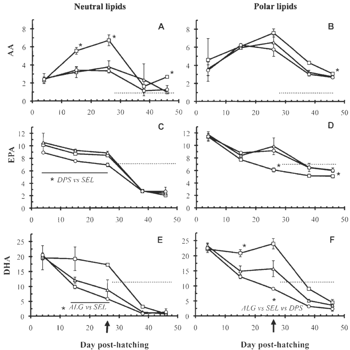
Figure I.1 Essential fatty acids (% of TFA \pm SD) in neutral and polar lipids in winter flounder larvae fed three rotifer enrichments ( \square AlgaMac 2000 [ ALG ], \triangle DHA protein Selco [ DPS ], \circ Selco 3000 [ SEL ]) until 26 dph then weaned onto non-enriched Artemia and a dry diet (Lansy Cw). Asterisks indicate significant differences in fatty acid content in the indicated treatment on a given sampling day. Arrows on the x-axes indicate the switch between rotifers and co-feeding and the horizontal dashed lines indicate the relative fatty acid level in the dry diet.
