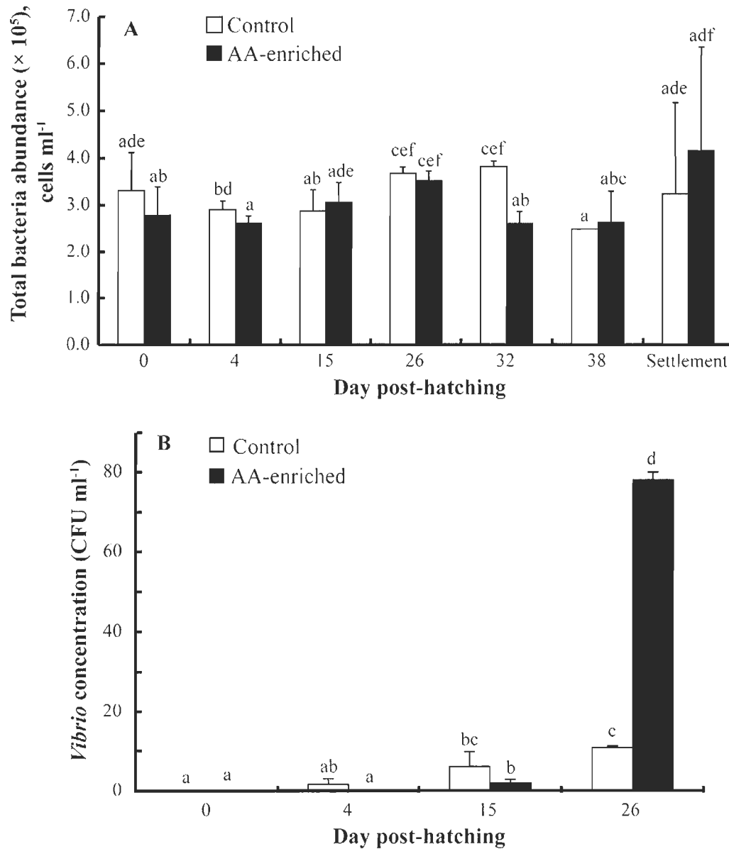
Figure III.4 A) Total bacteria abundance (cells ml -1 ± SD) determined using flow cytometry in control and AA-enriched larval tanks. B) Vibrio abundance (CFU ml -1 ± SD) in control and AA-enriched larval tanks. Different letters indicate significant differences among sampling times or diets.
