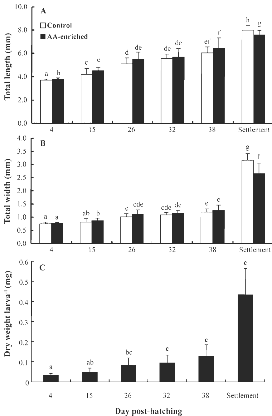
Figure III.1 Mean ( \pm SD) total length (A), width (B) and dry weight (C) of winter flounder larvae fed control and AA-enriched rotifers. Different letters indicate significant differences among sampling times or diets.
