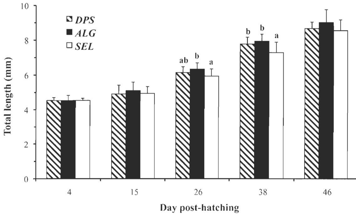
Figure I.2 Total lengths of winter flounder larvae fed three rotifer enrichment media (■ Algamac 2000 [ ALG ]; ▨ DHA protein Selco [ DPS ]; □ Selco 3000 [ SEL ]) until 26 dph and then weaned onto Artemia and a dry diet (Lansy Cw). Different letters indicate significant difference among larviculture treatments at a given day post-hatching.
