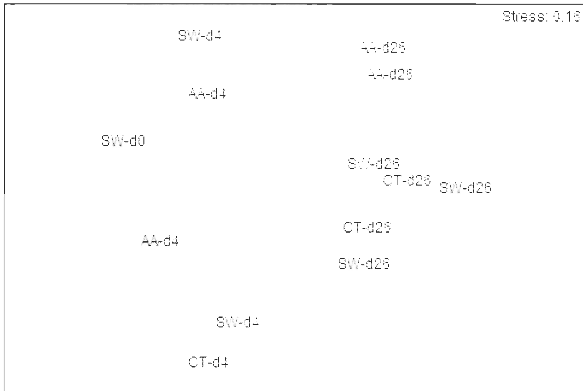
Figure III.5 NMDS diagram of the similarity matrix calculated from the binary DGGE data showing the changes in the bacterial community structure in larval rearing water. SW: source seawater (sampled prior to entering larval tanks), AA: water in AA-enriched larval tanks, CT: water in control larval tanks, d: sampling day.
