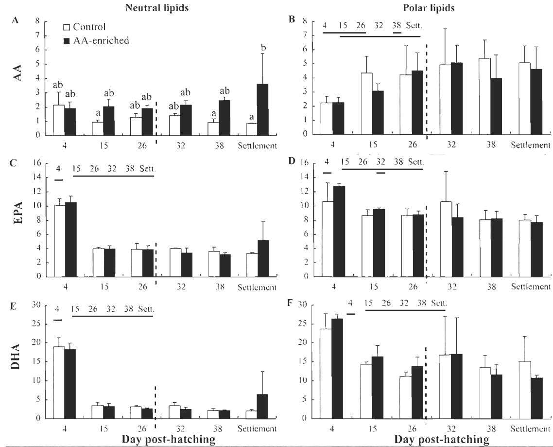
Figure III.2 Essential fatty acids (as percentage of TFA \pm SD) in winter flounder larvae fed control or AA-enriched rotifers. Different letters indicate significant differences among sampling times or diets. The results of the a posteriori tests are presented: solid lines underlie those days that are not significantly different one from the other.
