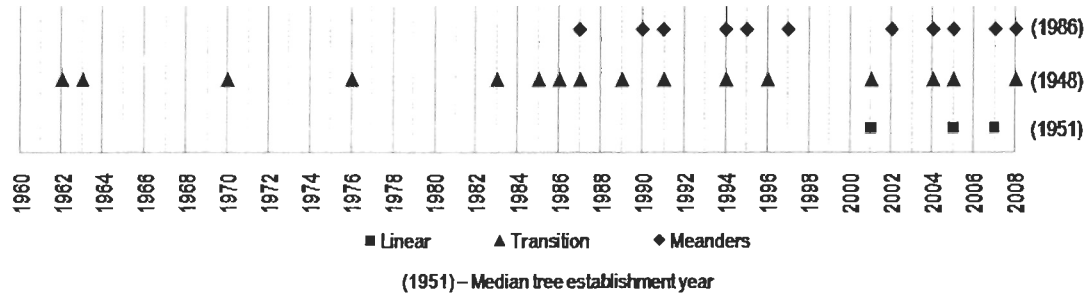
Figure 2.6 : Ice jam identification for the three morphologically distinct sections ■ : upstream linear; ▲ : transition; ◆ : meandering section. Year in parenthesis indicates median tree establishment year for each section.
