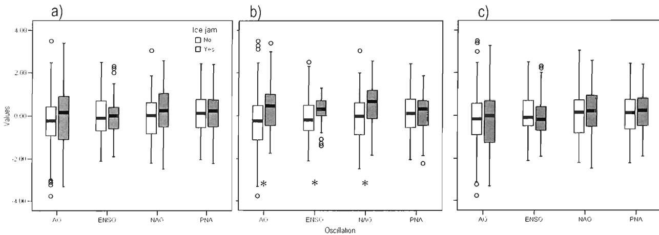
Figure 2.7 : Standardized large-scale oscillation values per sampling site AO : Arctic Oscillation ; ENSO : El Nino Southern Oscillation ; NAO : North Atlantic Oscillation ; PNA : Pacific Northern Oscillation. Vertical axis stands for standardized large-scale oscillation values. Boxes represent the interquartile range, bold line median value, circles values more than 1.5 to 3 box lengths. Significantly different boxplots between jam years and non jam years per oscillation are indicated with *. A) Both sites; B) Meanders and C) Transition
