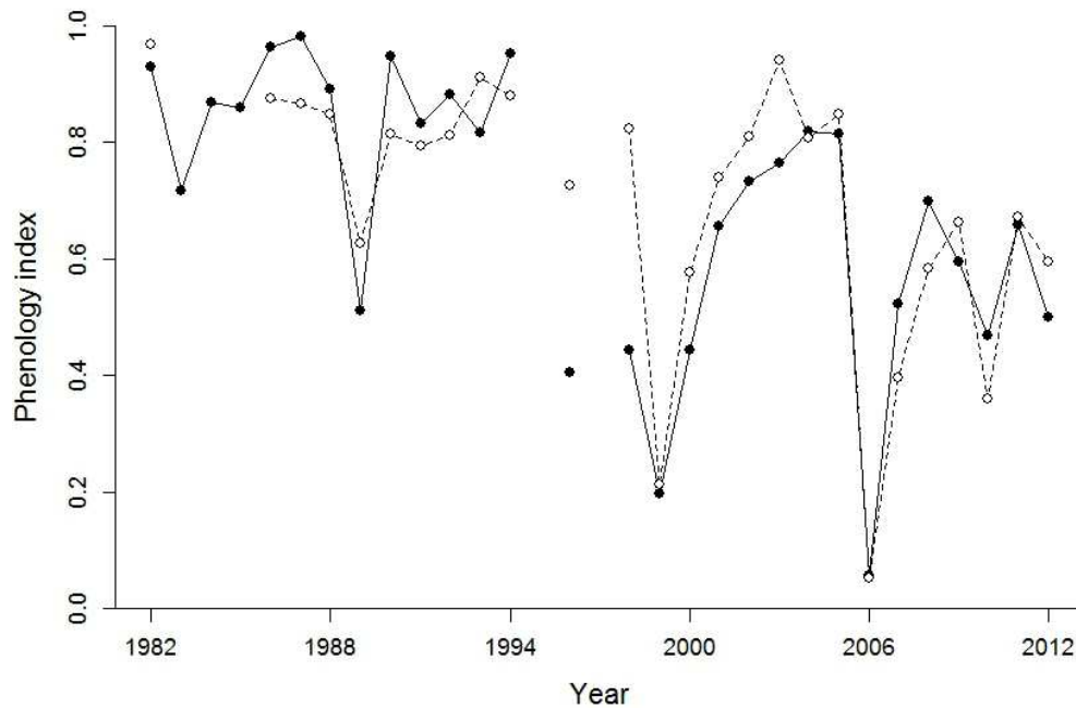
Figure 2.2 Phenology indices of larval snow crab (full line, black circles) and toad crabs (dashed line, white circles) in the southern Gulf of St. Lawrence from 1982 to 2012. Phenology indices were calculated using the proportions of zoea 1 by taxon in each year (see methods) and ranged from 0 to 1, with low and high index values indicating respectively late or early phenology.
