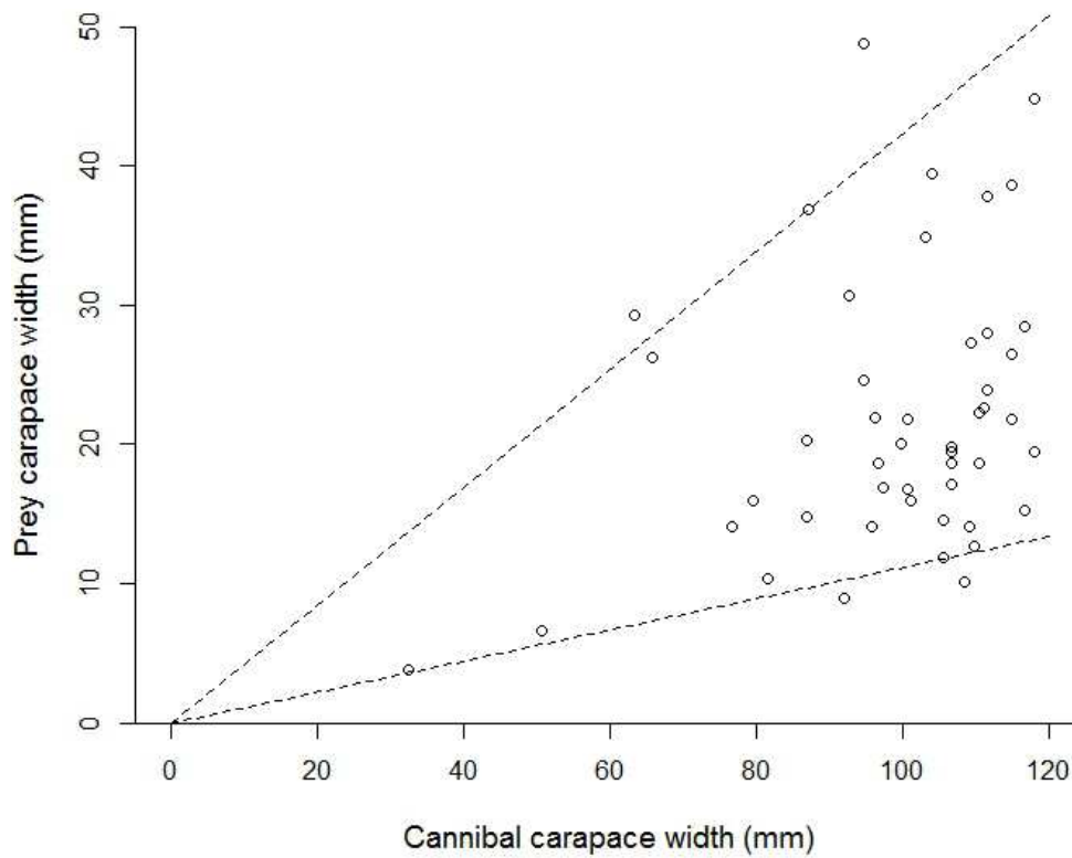
Figure B.3 Prey carapace width plotted against cannibal carapace width based on stomach contents of wild caught male snow crabs from the estuary and northwest Gulf of St. Lawrence (source: Lovrich et Sainte-Marie, 1997). Dotted lines indicate the assumed upper and lower limit of prey carapace width for a given cannibal carapace width.
