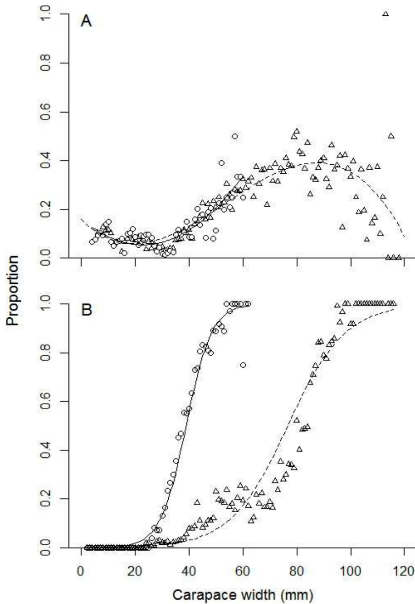
Figure 3.2 Proportion of skip-molters (A) and of terminally molted crabs (B) by 1-mm carapace width interval, and the fitted polynomial and logistic equations for female ( \circ , black full line) and male snow crabs ( \Delta , black dashed line). Data come from a trawl survey conducted each year since 1989 by the Department of Fisheries and Oceans to monitor the snow crab population in Baie Sainte-Marguerite, eastern Canada. The polynomial and logistic equations were used to estimate the probabilities of skip-molting and undergoing terminal molt, respectively.
