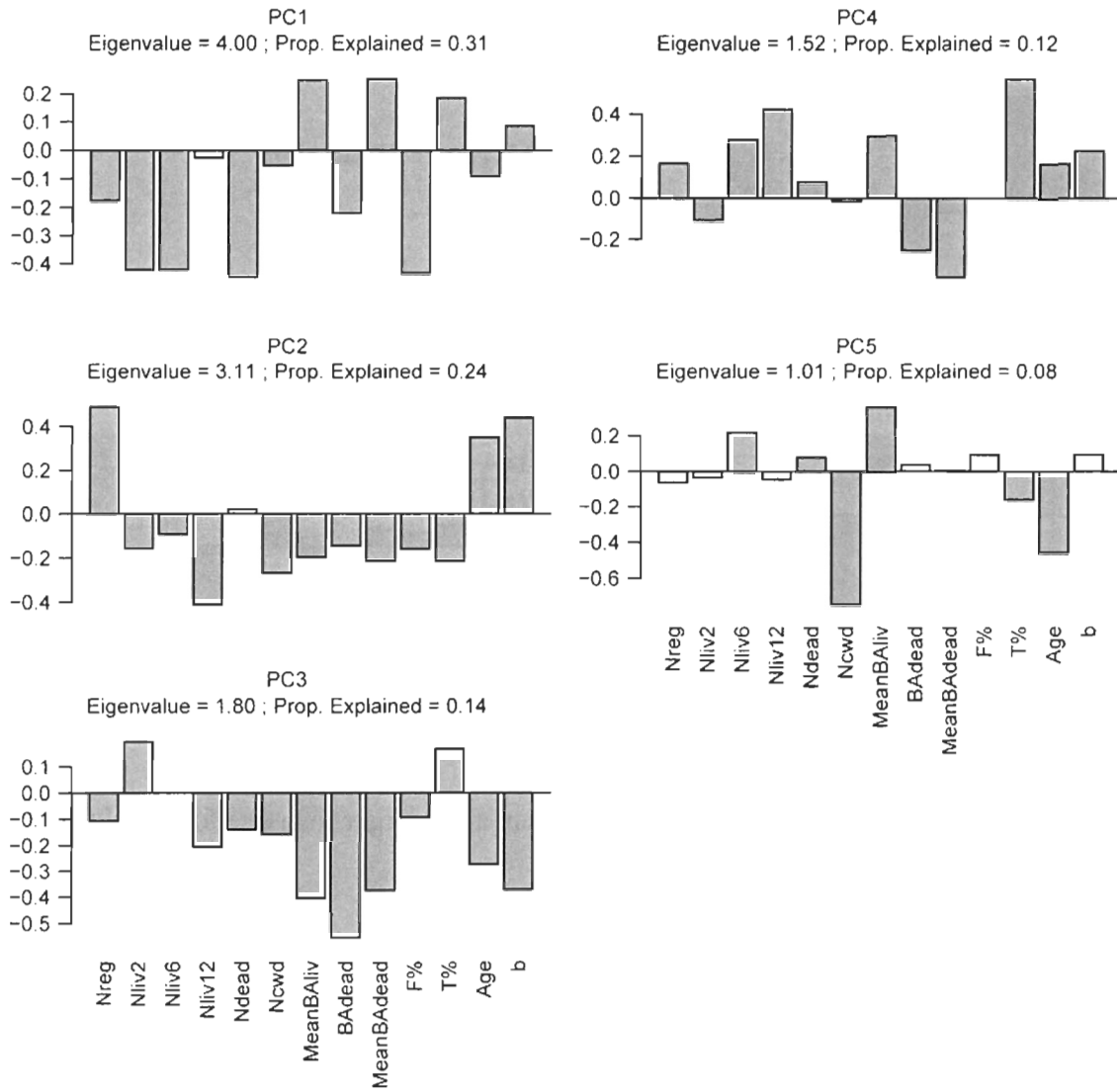
Fig. 2.S2. Loadings of components with eigenvalues larger than one for L18 PCA.
