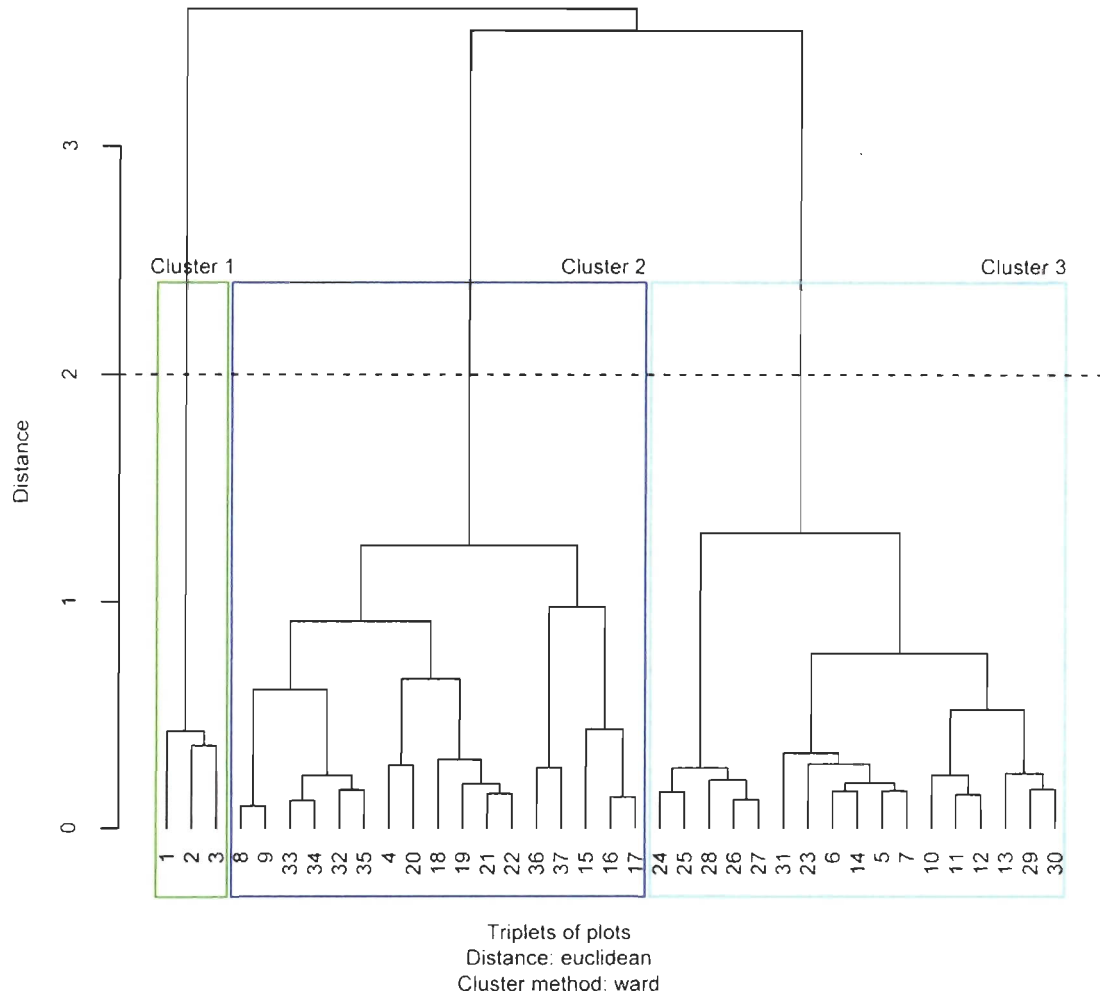
Fig. 2.S6. Cluster dendrogram for L18 triplets of plots. The horizontal dashed line shows the threshold used to define homogeneous clusters.
