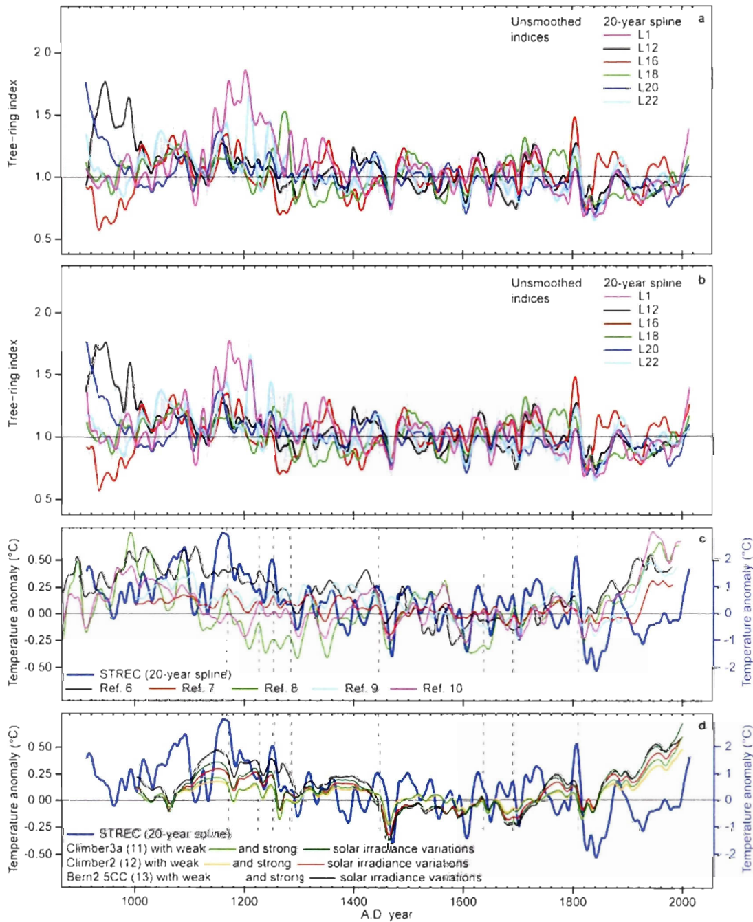
Fig. 3.S3. The network of millennial-long tree-ring chronologies and comparison between STREC and Northern Hemisphere records used in the IPCC-AR4. The two top panels show the six local RCS chronologies (one per lake and composed of living and subfossil trees) over the 1102 years retained for STREC before (a) and after (b) the reconstruction of the non-robust time intervals (i.e. intervals for each local chronology where the R_{bar} statistic calculated over the 31-year moving windows is
