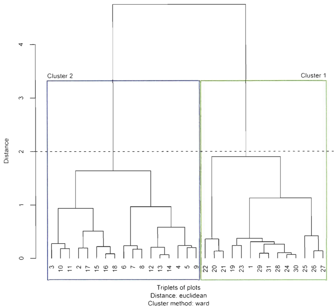
Fig. 2.S7. Cluster dendrogram for L20 triplets of plots. The horizontal dashed line shows the threshold used to define homogeneous clusters.
