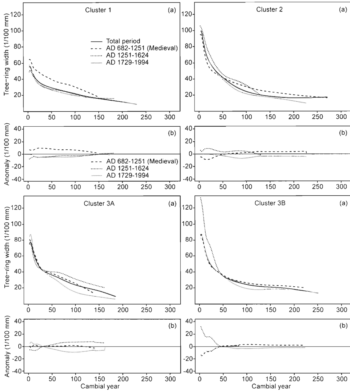
Fig. 2.S9. Comparison among fire-free intervals of the smoothed average growth curves of the subfossil logs for each cluster at L18. The "a" plots show the smoothed average growth curves, while the "b" plots show the growth anomalies calculated with a subtraction against the average of the three curves (curves for the periods 682-1251, 1251-1624 and 1729-1994). The legends in the plots of the first cluster also refer to the other plots.
