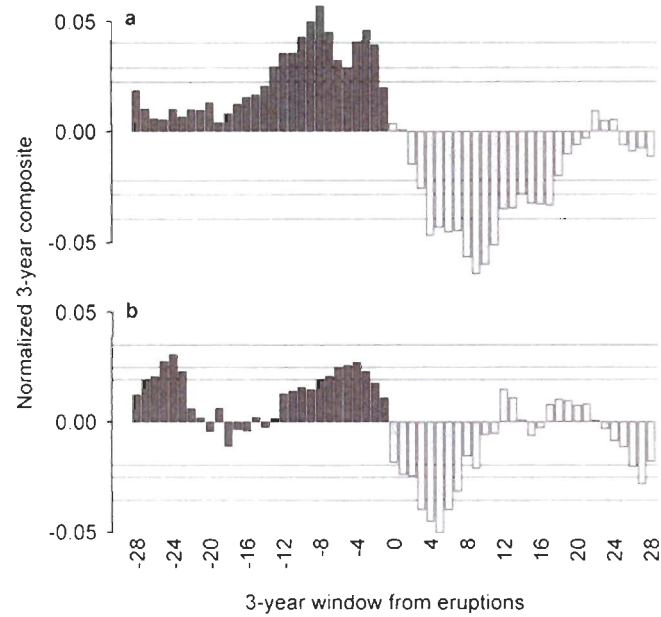
Fig. 3.3. STREC responses to volcanic eruptions. Dimensionless normalized 3-year composites which are the result of the Superimposed Epoch Analysis showing summer temperature responses in Eastern Canada to the 10 strongest (a) and 10 strong (b) volcanic eruptions of the last millennium deduced by ref. 9 (see SI Methods). Each 3-year composite is labeled with the year nearest to the eruption year (e.g. 0 stands for the 3-year composite composed of years 0, 1, and 2 from eruption). Confidence ranges (90%, 95%, 99%) are indicated by horizontal lines. Black and grey columns mark pre and post eruption composites.
