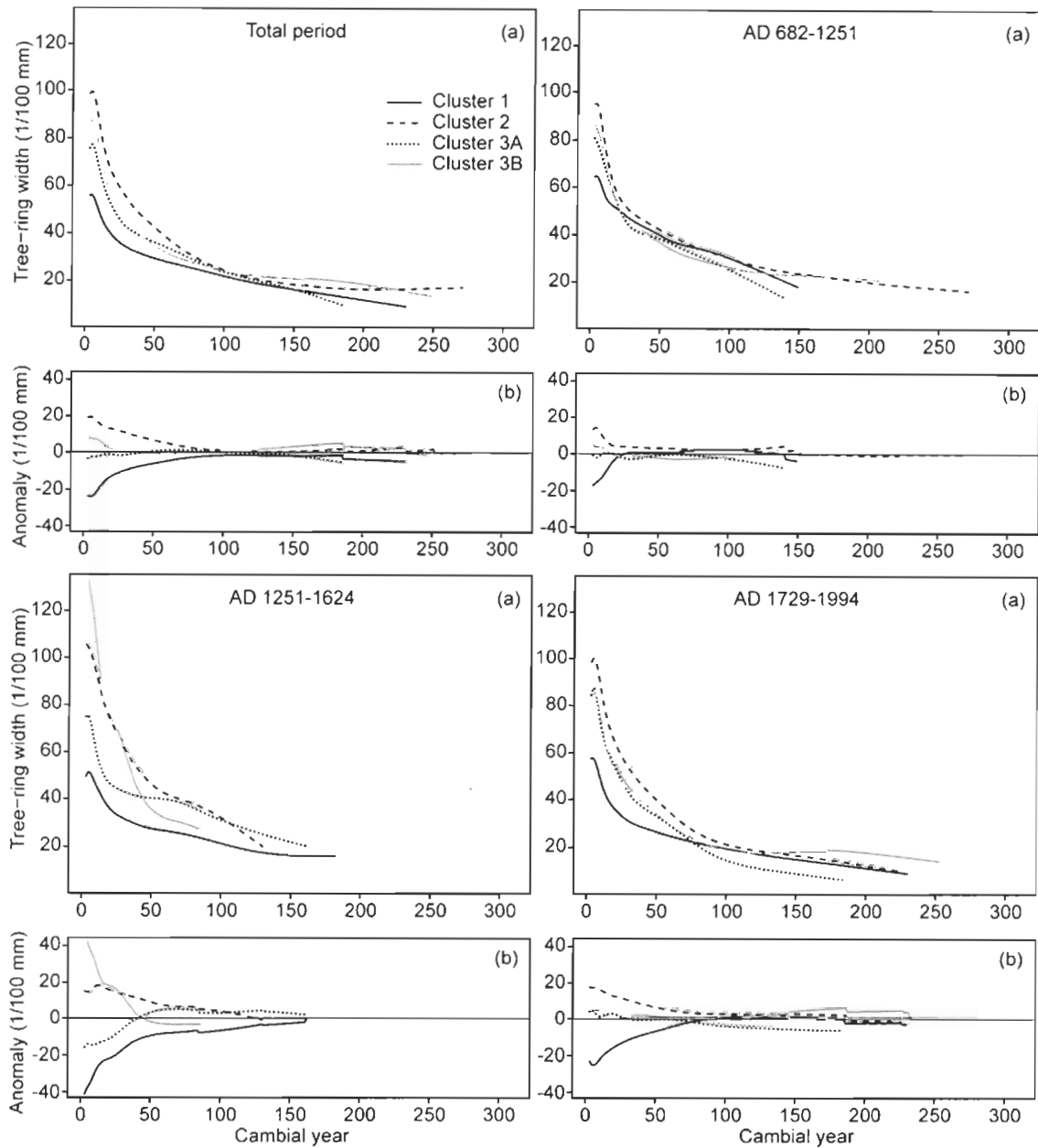
Fig. 2.6. Comparison among all clusters at L18 of the smoothed average growth curves for the subfossil logs recruited during different fire-free intervals. The "a" plots show the smoothed average growth curves, while "b" plots show the growth anomalies calculated with a subtraction against the average of the four curves with each corresponding to a cluster or a cluster section. The legend in the first "a" plot refers to the other plots as well.
