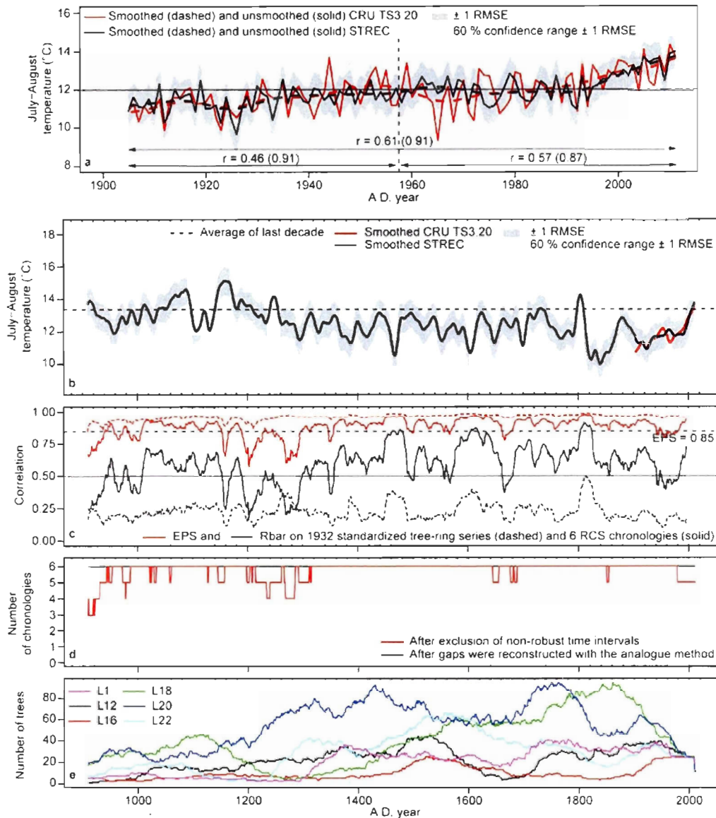
Fig. 3.1. STREC reconstructed values and robustness. Observed (15 cells of the CRU TS3.20 dataset covering our sampling sites) and reconstructed (STREC) July-August temperatures in the taiga of Eastern Canada during the last century (a) and the last 1100 years (b). Smoothed values are 20-year splines. In a, correlations between brackets refer to smoothed values. Expressed Population Signal (EPS) and Rbar statistics computed over 31-year moving windows are also shown (c), as well as replication among (d) and within (e) chronologies.
